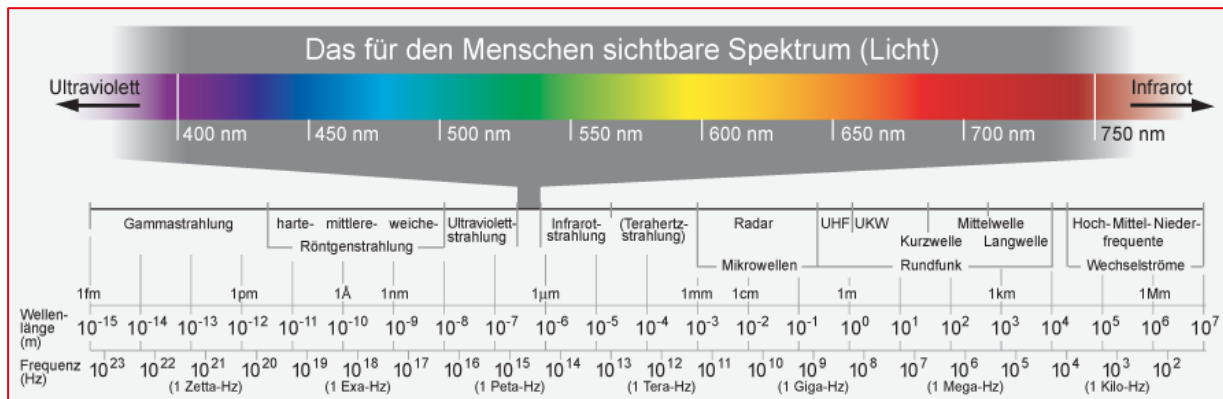
Electromagnetic Radiation Wavelengths and Frequencies
